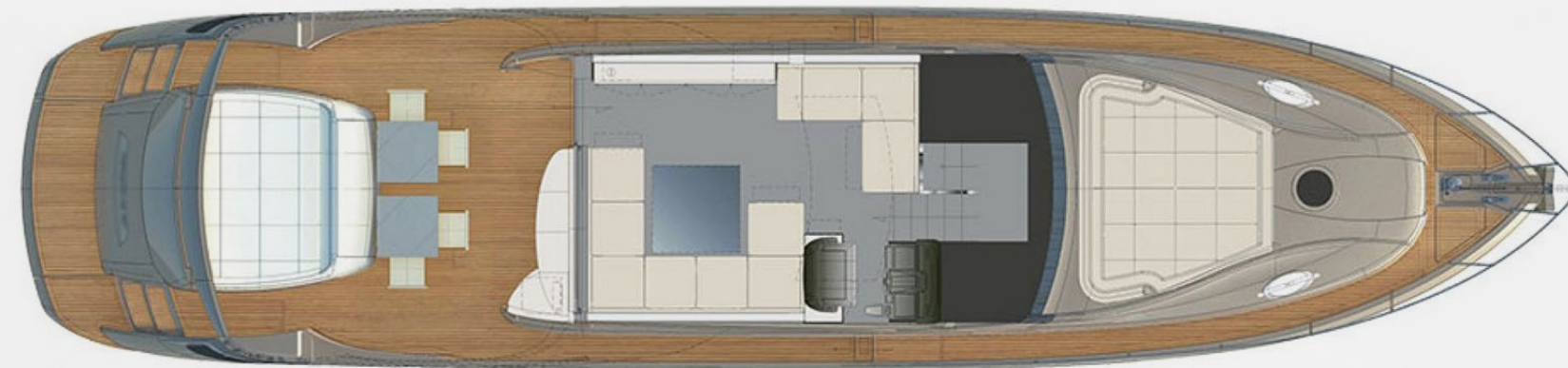
MAIN DECK
